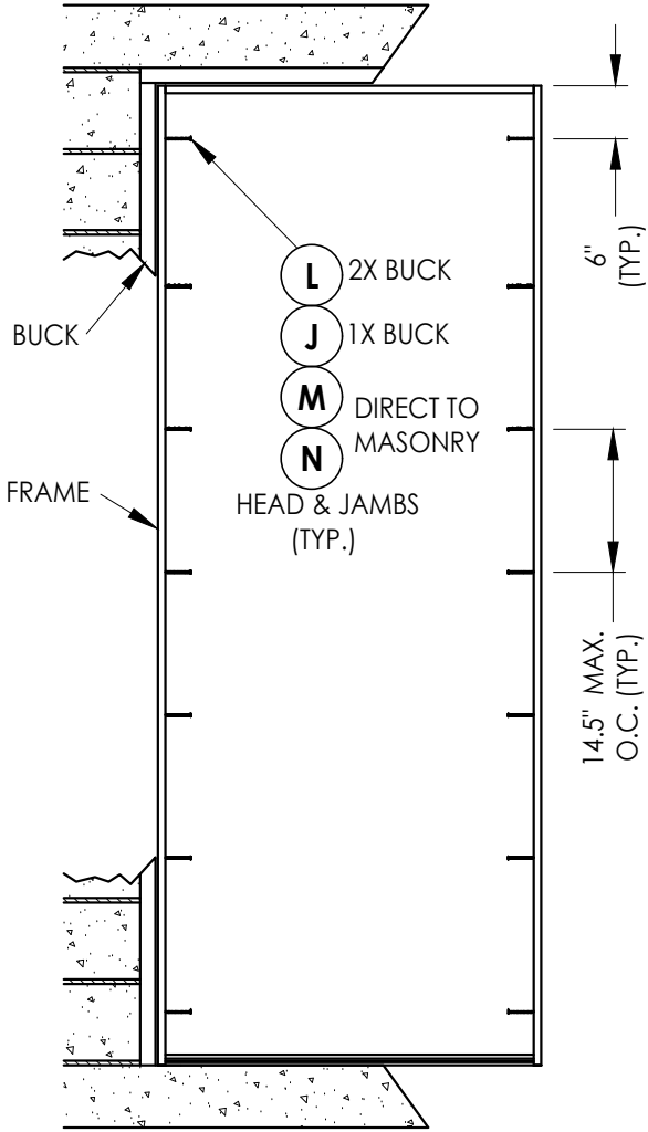
FRAME ANCHORING
